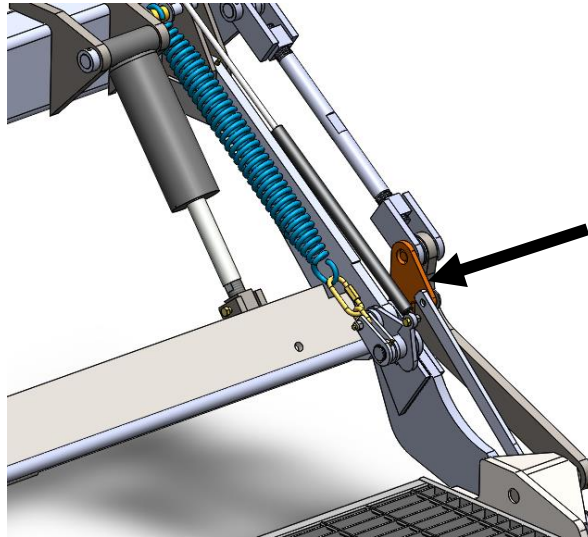
Right Hand Fold Link Assembly
