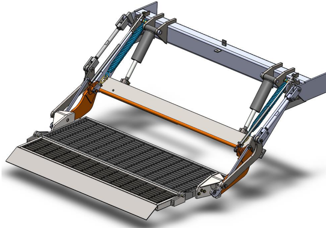
CA-803-120 (complete with bearings)
