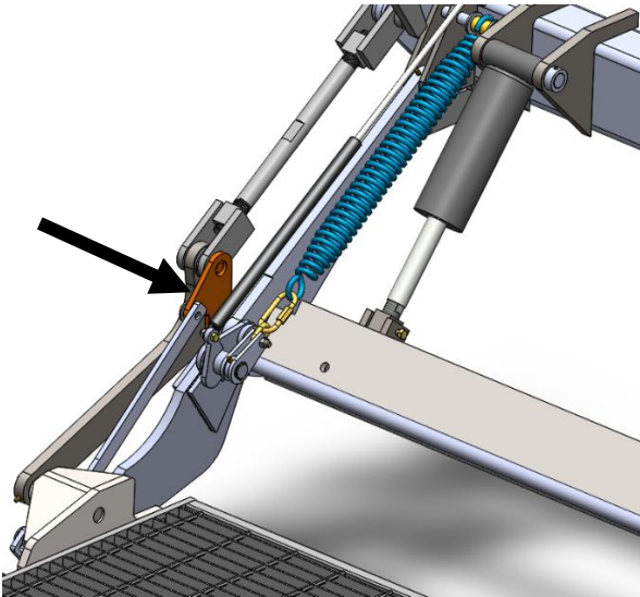
Left Hand Fold Link Assembly
